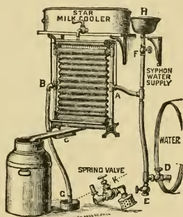
Star Milk Cooler.
